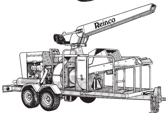
(SHOWN WITH OPTIONAL FORWARD PLATFORM AND TANDEM AXLE CONFIGURATION)
